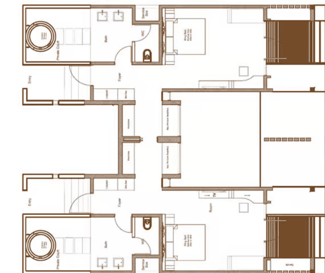
Family Bungalows - 138 SQM 2
